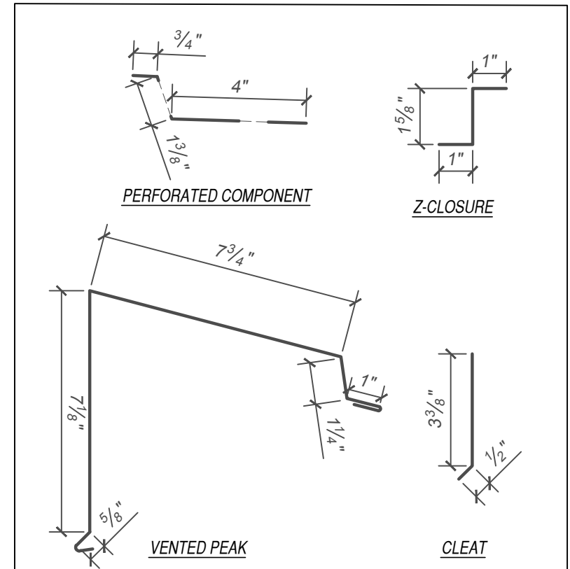
FLASHINGS
