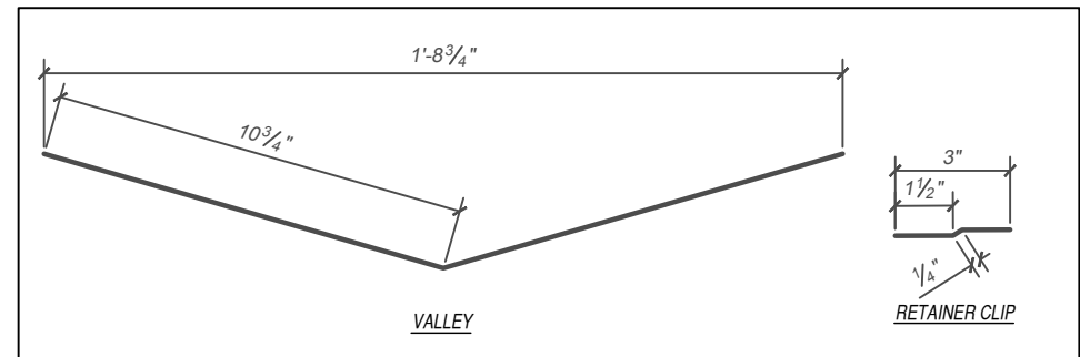
FLASHINGS
