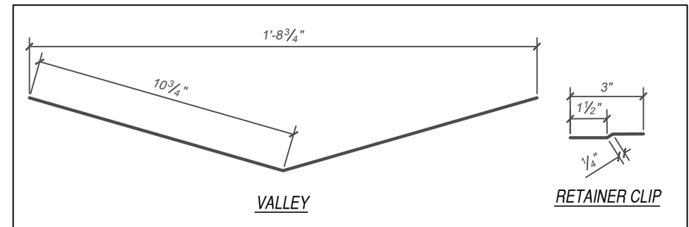
FLASHINGS
