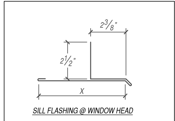
FLASHINGS
