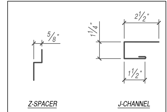
FLASHINGS
