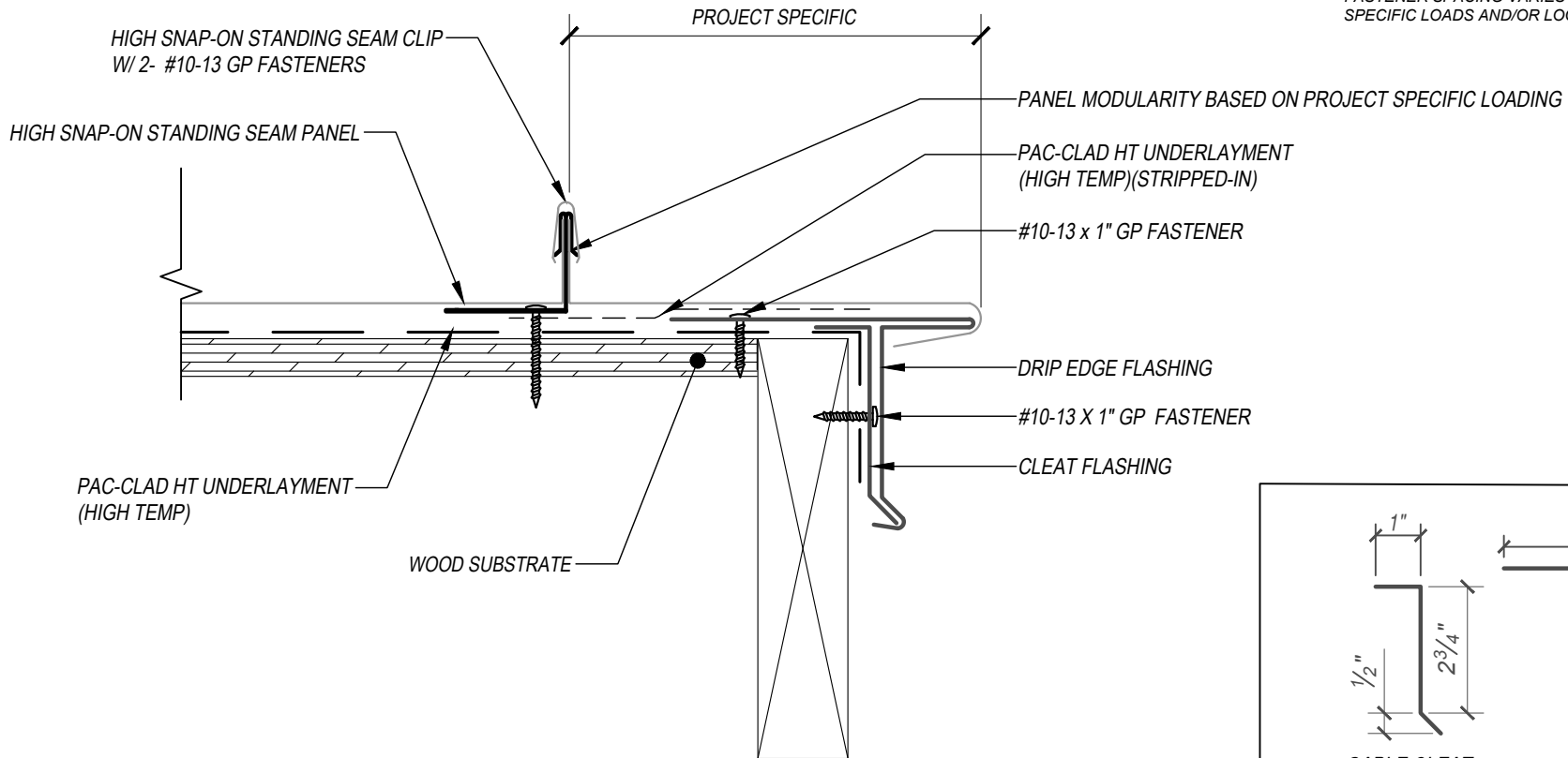
FLASHINGS
