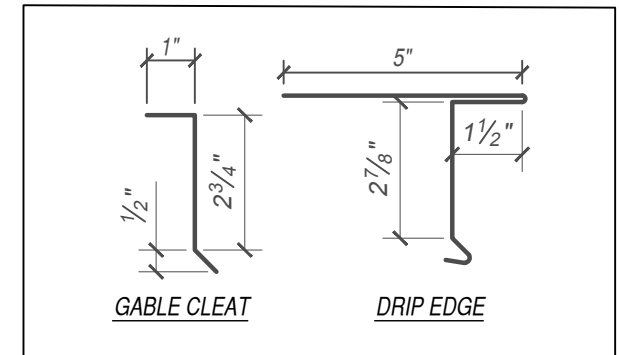
FLASHINGS
