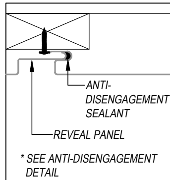
REVEAL ANTI-DISENGAGEMENT OPTION
