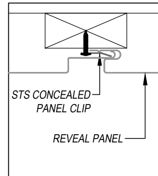
REVEAL CONCEALED CLIP OPTION
