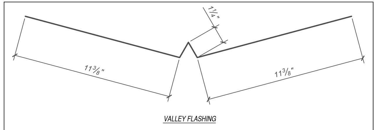
FLASHINGS
