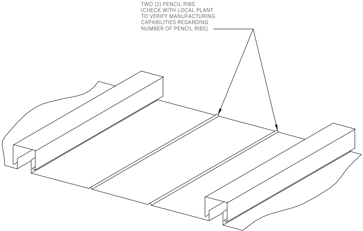
SNAP-ON BATTEN PANEL WITH PENCIL RIBS ISOMETRIC VIEW
