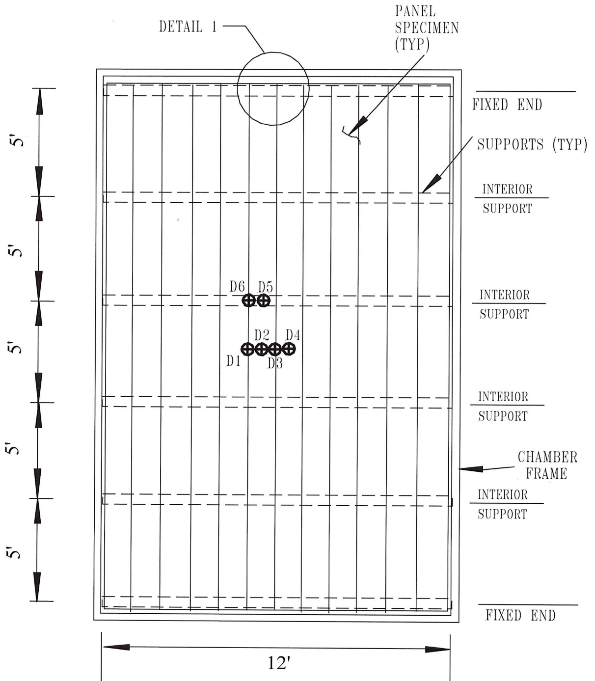
PLAN VIEW
